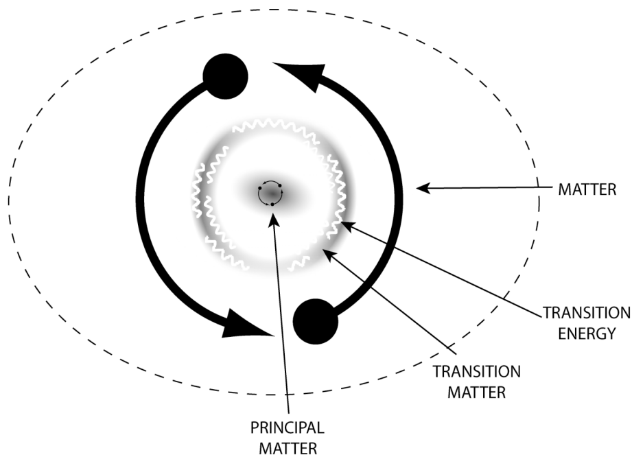
Fig. 11 The magnetic field structure of the plasma of the light
