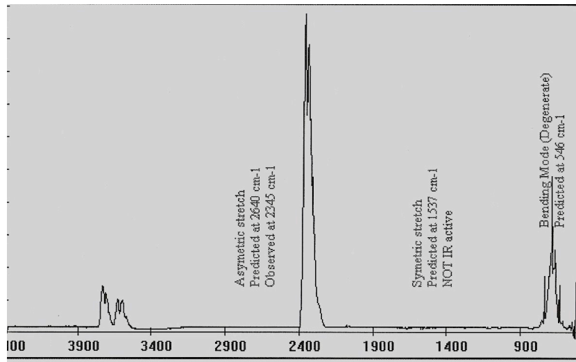
Fig. 22 Standard CO2 infrared spectroscopy graph.
