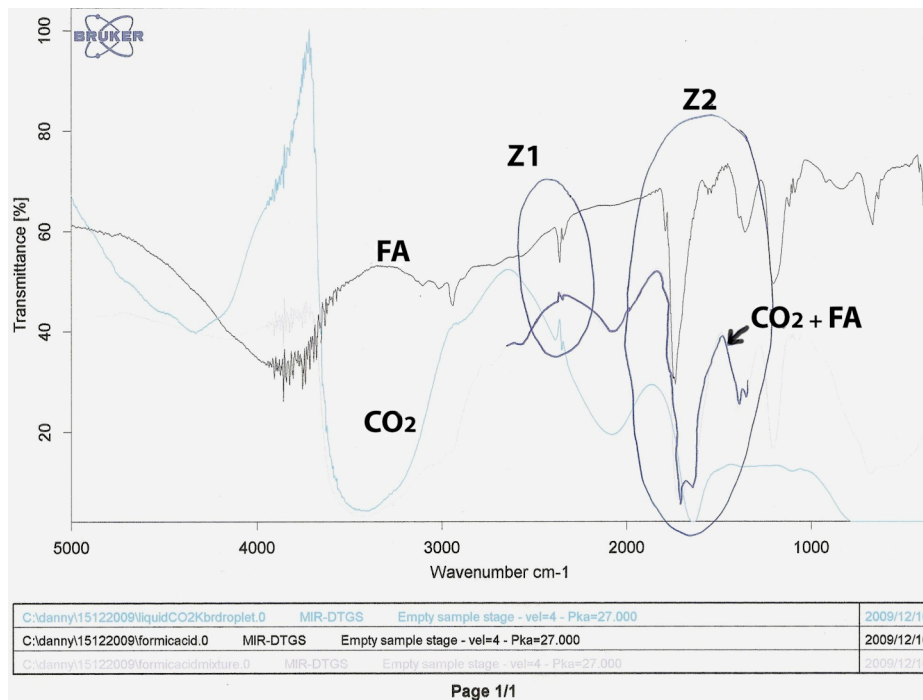
Fig. 28 The superimposed graph of CO 2 and conversion o Formic acid and formic acid and mixture of formic acid and solution of nano CO 2 .
