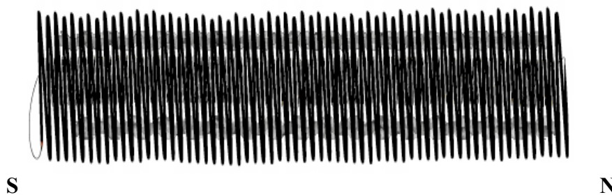
Fig. 4 The polarity of the ray of light
