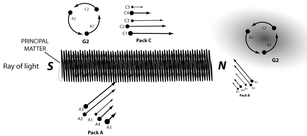
Fig. 10B Ray of light travelling through and interacting with outer mafs and initial fundamental particles of pmfs.
